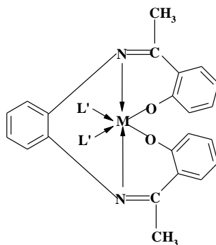
Figure-1: Proposed octahedral geometry of investigated Co-complexes
