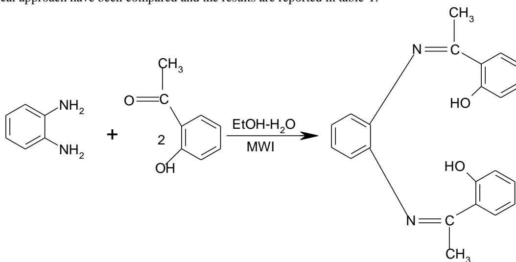
Scheme-1: Microwave assisted synthesis of ligand
