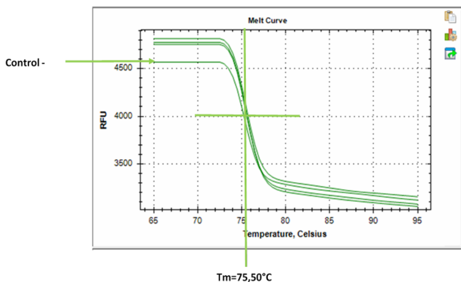
Figure 3. Melting curves of the 28S CMA gene in real-time PCR.
