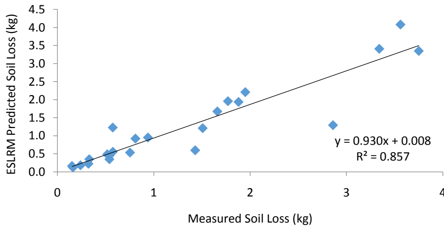
Figure. 2: Verification of Measured and Predicted Soil Loss Using Empirical Model for other 23 test
