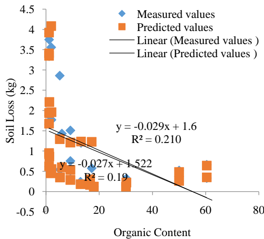
Figure 11: Verification of Soil Loss and Organic Content (%)
