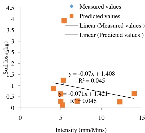
Figure 9: Calibration of Soil Loss and Intensity (mm/mins)
