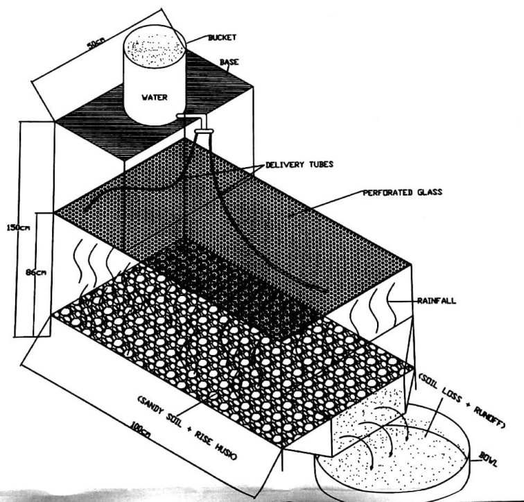
Figure 2: Diagram of a Rainfall Simulator
