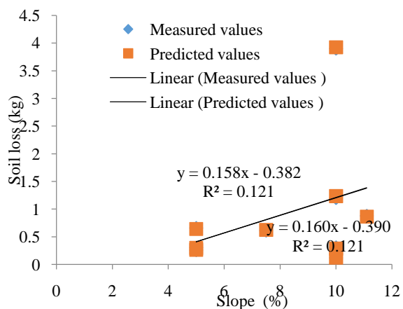
Figure 8: Calibration of Soil Loss and Slope (%)
