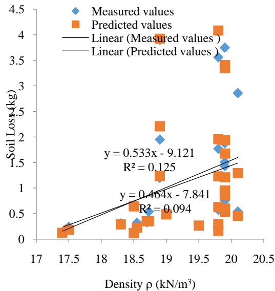
Figure 13: Verification of Soil Loss and Density \rho (kN/m 3 )
