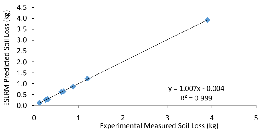
Figure. 1: Calibration of Measured and Predicted Soil Loss Using Empirical Model (ESLRM)
