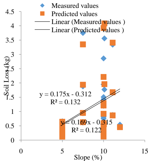
Figure 15: Verification of Soil Loss and Slope in percentage
