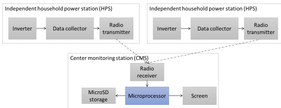
Figure1. System diagram
