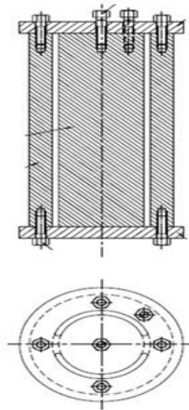
Figure 1. Sensor design
