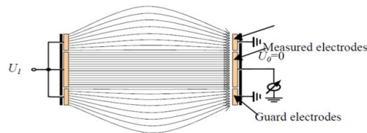
Figure2: three terminal electrodes
