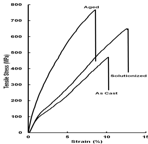
Fig.1 Tensile stress-strain plots of the bronze samples in as cast and heat treated conditions
