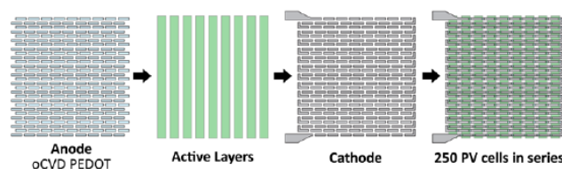
Fig. 1 The diagram shows how the researchers create an array of interconnected PV cells. Using their masking technique, they first lay down the anodes; next come the active layers at a 90-degree angle; and finally the silver cathodes—a little offset from the anodes so as to connect each cell to the one next to it. Little L’s connect the end of one row to the beginning of the next.
