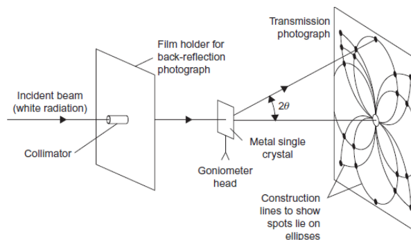
Figure.7:Schematic shows Laue method [1].
