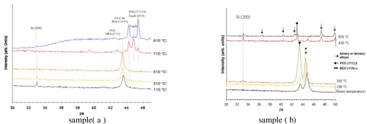
Figure.12: XRD patterns of two samples evaluate their behavior during annealing.
