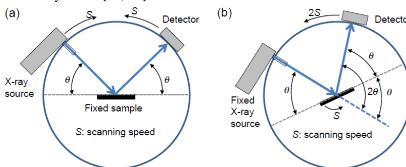
Figure.6: Schematic shows the types of XRD Goniometers, (a) θ-θ type, (b) θ- 2θ type [14]
