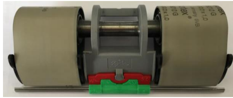
Fig.3. Active Cradle with roller, top apron, clip and pressure bar.
