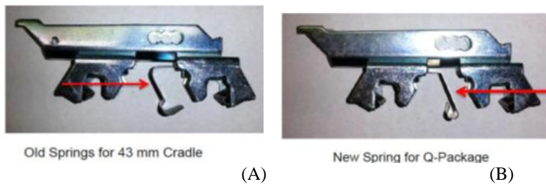
Fig.7. Old springs (A) and new spring (B).
